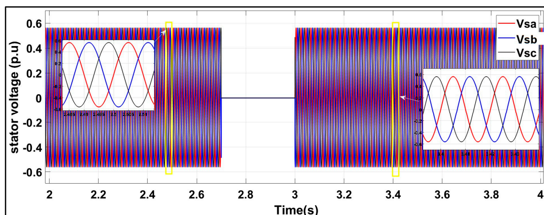
Figure 13. Three-phase stator voltage under a symmetrical fault with the conventional scheme.
