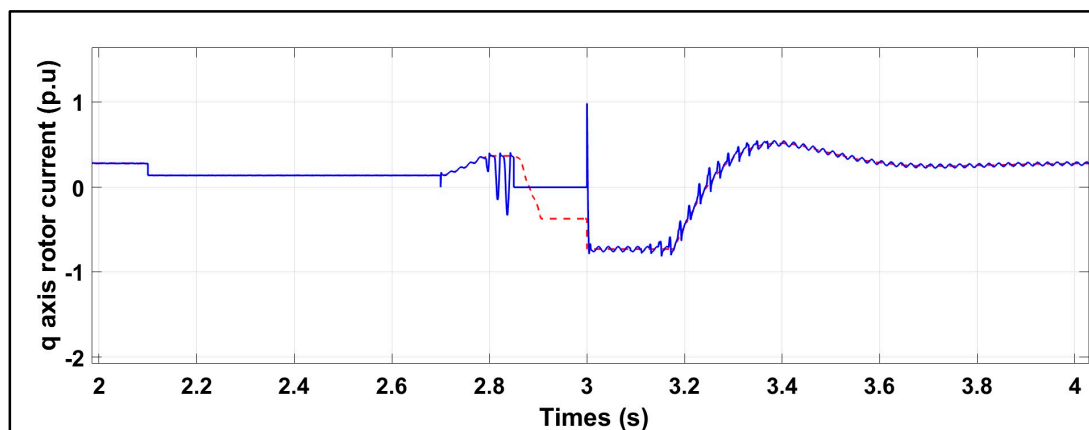
Figure 20. q axis rotor current under a symmetrical fault with the proposed control scheme.
