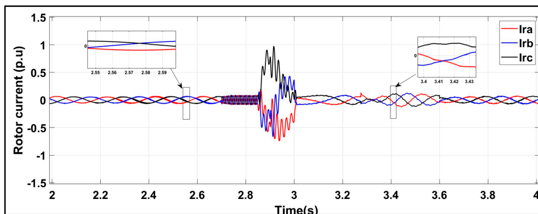
Figure 19. Three-phase rotor current under a symmetrical fault with the proposed control scheme.
