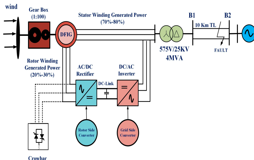
Figure 5. DFIG-based wind turbine under simulation study with fault.
