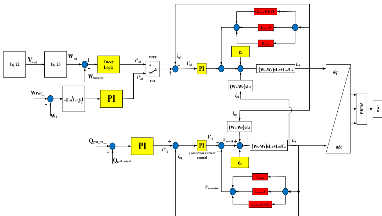
Figure 4. Proposed modified rotor current control scheme.
