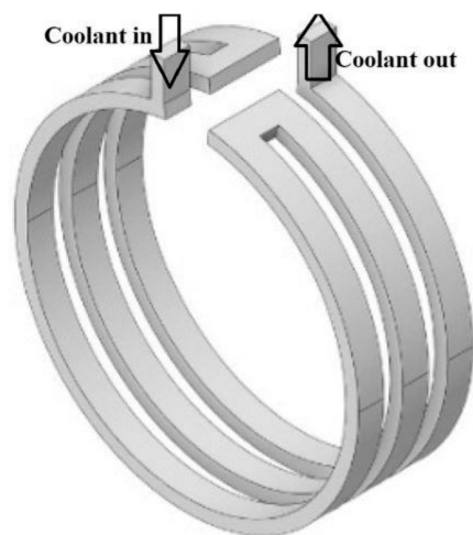
Figure 10. Tangential water flowing through the induction motor housing [45].
