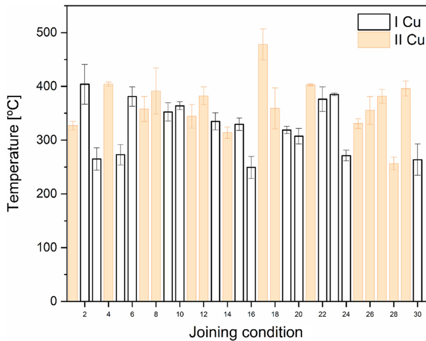
Fig. 5 – Peak process temperatures of 30 joining conditions used to produce joints of AA-2024-T3 rivet and different FR4 material configurations (I Cu and II Cu) according to BBD, see Table 1.
