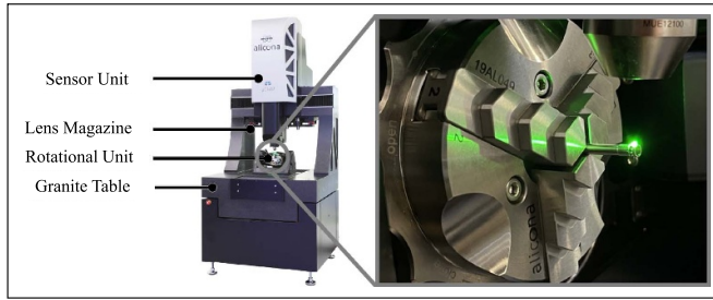
Figure 5. Inline setup of the focus variation. Reproduced with permission from [18].
