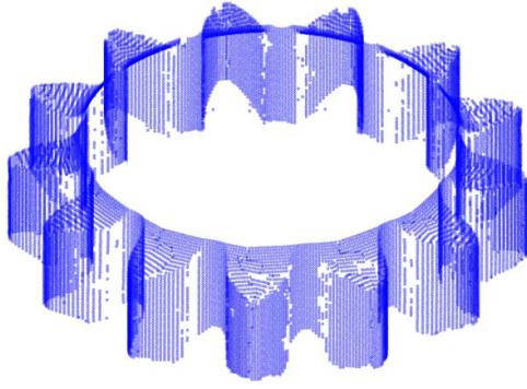
Figure 6. Full gear measurement.
