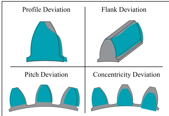
Figure 2. Geometric gear deviations, including profile, flank, pitch, and runout errors. Reproduced with permission from [11].
