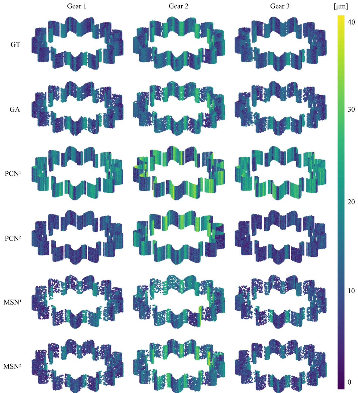
Figure 9. Distances to the master geometry from predictions in \mu\text{m} .
