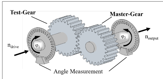
Figure 3. Setup of a single-flank rolling test, where the test gear rolls against a master gear. Angular deviations are recorded to determine the transmission error. Reproduced with permission from [5].
