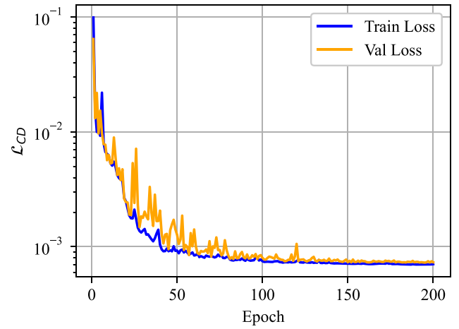
Figure 8. Train and validation loss curves for the MSN model using \mathcal{L}_{CD} for training.
