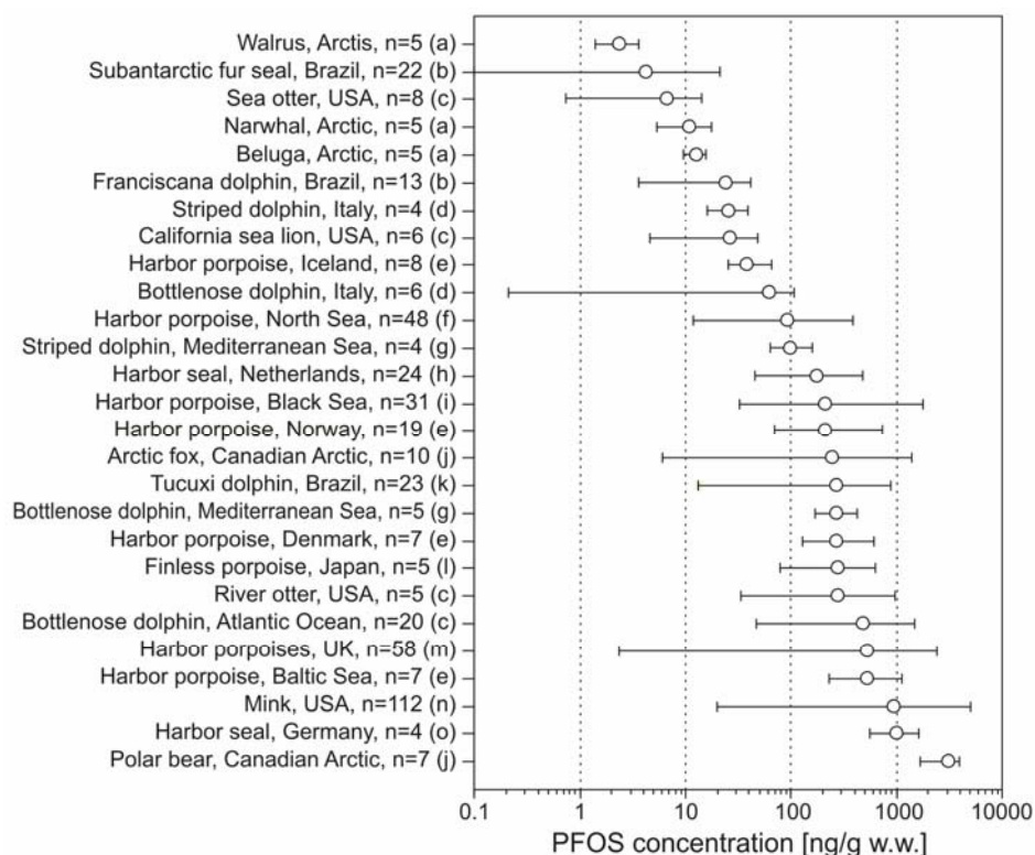
Figure 5. Hepatic concentrations (minimum, maximum, mean (circles)) of PFOS in mammals from (a) Tomy et al. 2004a, (b) Leonel et al. 2008, (c) Kannan et al. 2001b, (d) Kannan et al.
